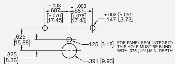
Mounting Detail
