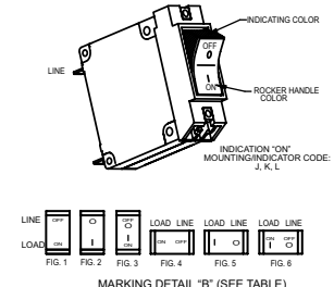
MARKING DETAIL "B" (SEE TABLE)
