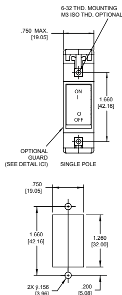
Panel Mounting Detail Mounting Detail Tolerance: ±.005 [.13] unless noted
