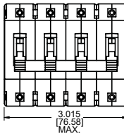
Panel Mounting Detail Tolerance ±.005 [.13] unless noted.
