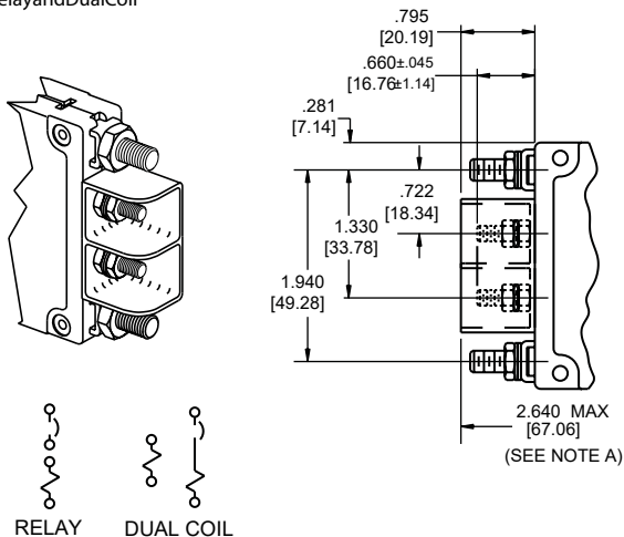
RelayandDualCoil
