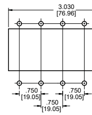
Mounting Detail*
