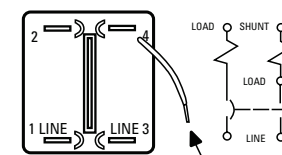
Two Pole (1 pole shunt)
