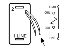
Relay Trip (Note A) Single Pole
