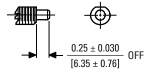
Push-to-Reset Actuation (Single and Two Pole)
